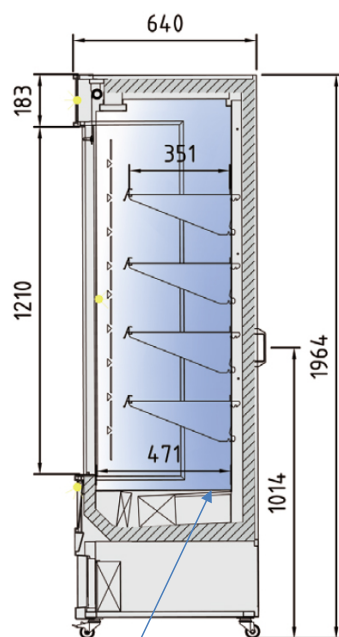
TEMPERATURE SENSOR
