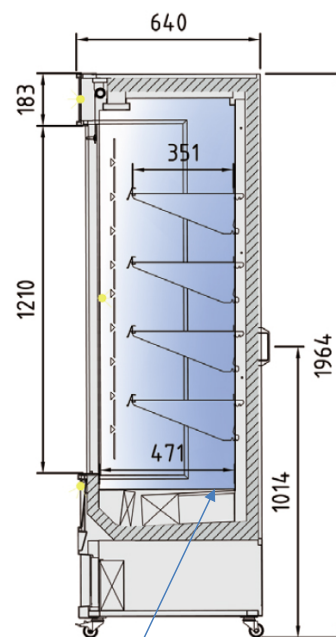
TEMPERATURE SENSOR
