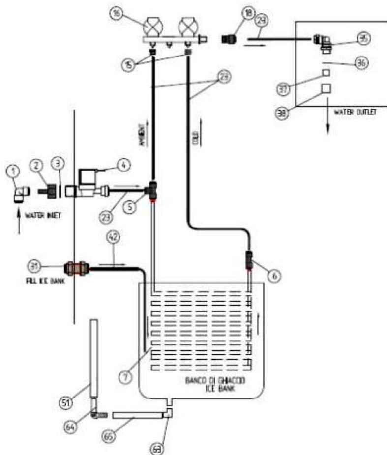
Aquality/Model A 20 IB AC Hydraulic Diagram
