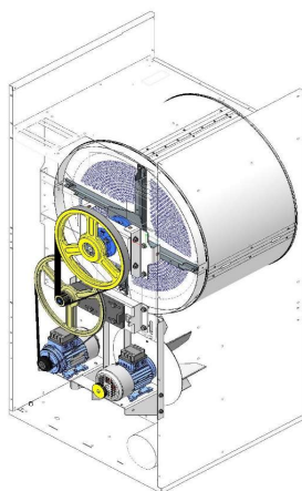
TRASMISSIONE TRANSMISSION
