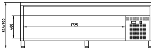
Dimensions (mm)
